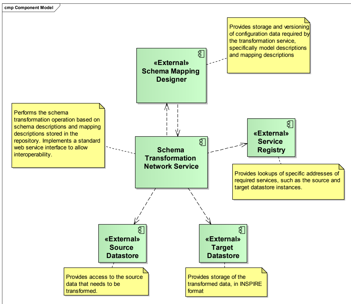
Figure 5 Component Model
