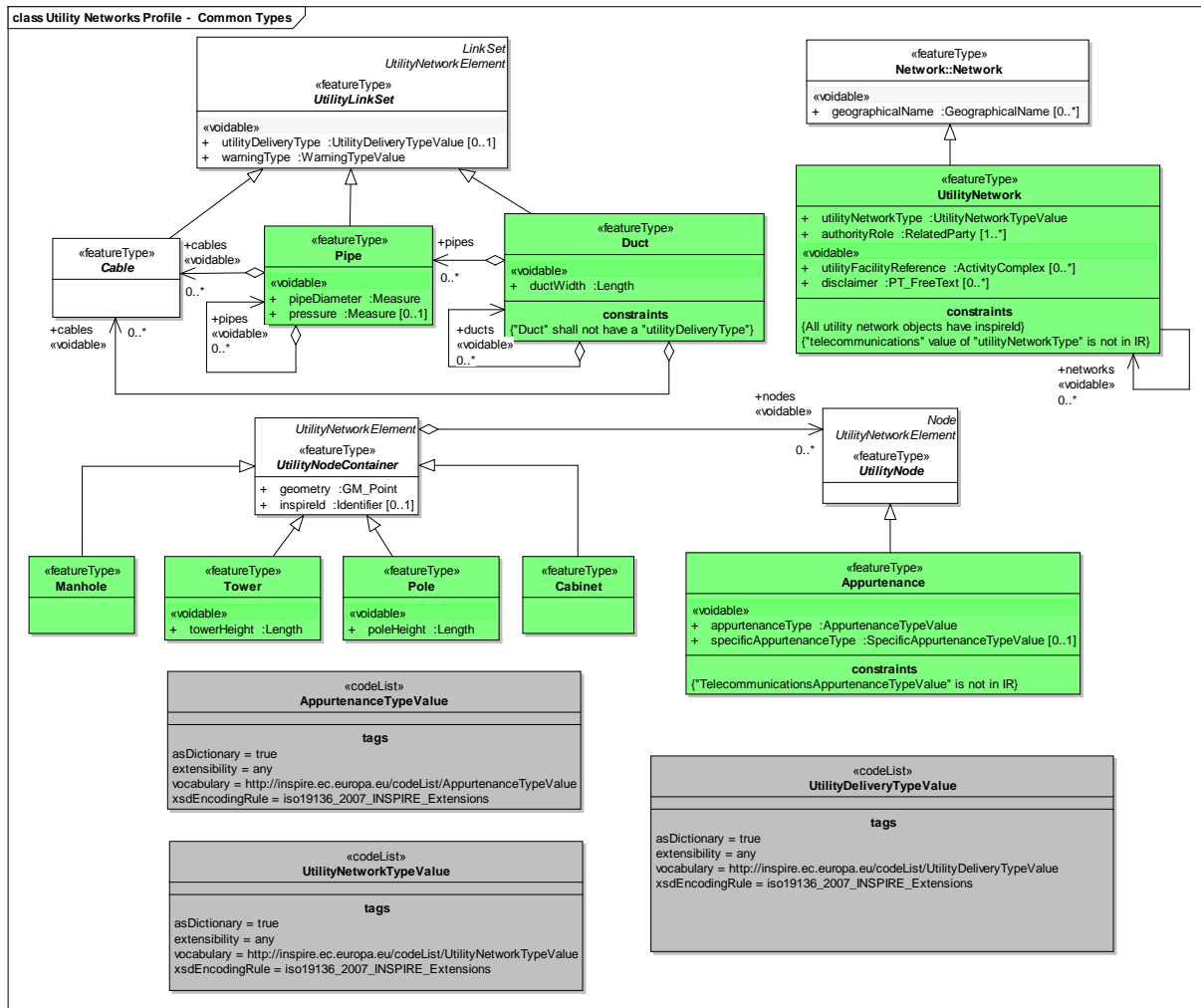
Figure 11 – UML class diagram: Overview of the “Utility Networks Profile - Common Types”
