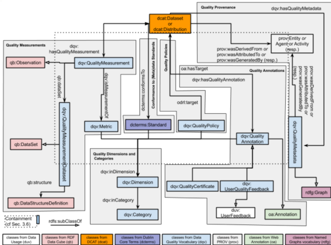
Fig. 1. Diagram depicting DOV classes and properties. For the sake of readability, the diagram does not include all the DOV properties.
